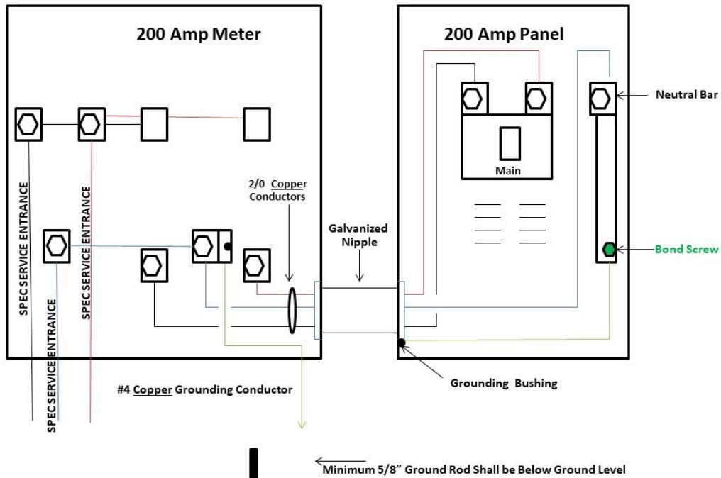
200 Amp UnderGround Meter Loop with Galvanized Nipple
